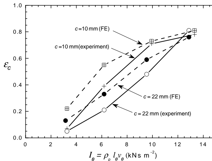
Fig. 6. Measured permanent core compression \varepsilon_c at the mid-span of the dynamically loaded sandwich plates, as a function of the initial foam projectile momentum I_0 . Finite element (FE) predictions (rate dependent model) for \varepsilon_c are included.
