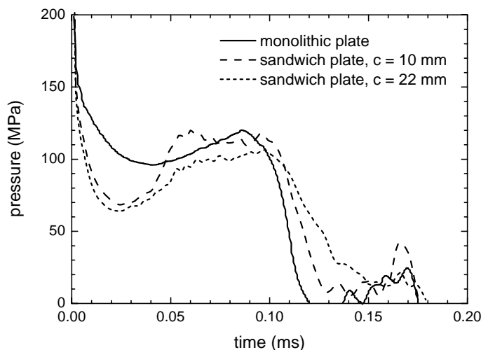
Fig. 12. The predicted pressure versus time histories exerted by the foam projectiles on the monolithic specimen M9, and the sandwich plate specimens A4 ( c = 10 mm) and B4 ( c = 22 mm). I_0 = 13 \text{ kN s m}^{-2} .
